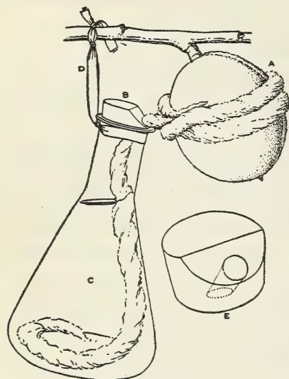
FIG. 6.—Device for supplying moisture for outdoor inoculations: A , Wick of absorbent cotton; B , cork; C , water container; D , attachment to host; E , enlargement of B . ( A to D are about one-half natural size.)
